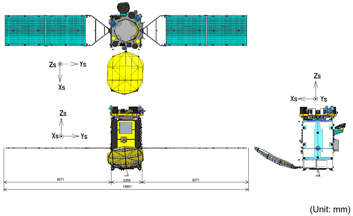
Figure 4 Satellite dimensions
