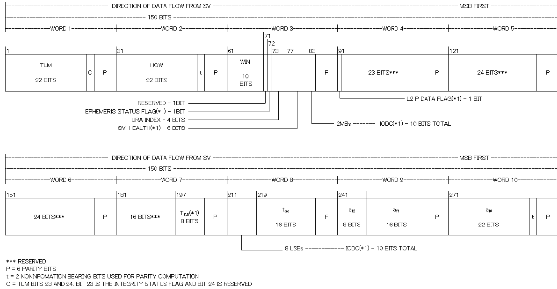
Figure 4.1.2-2 Subframe 1 Format
