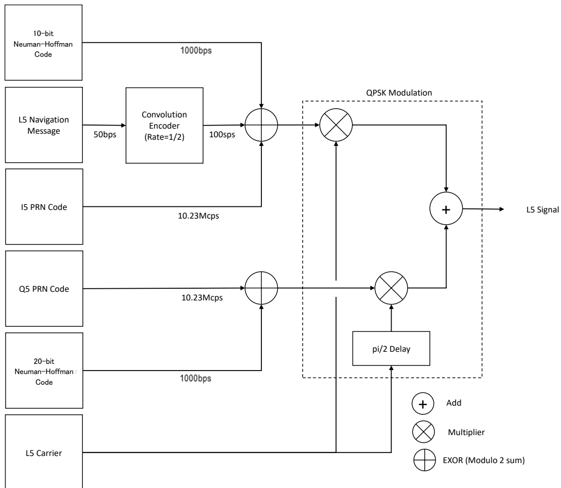
Figure 3.1.3-6 L5 Modulation
