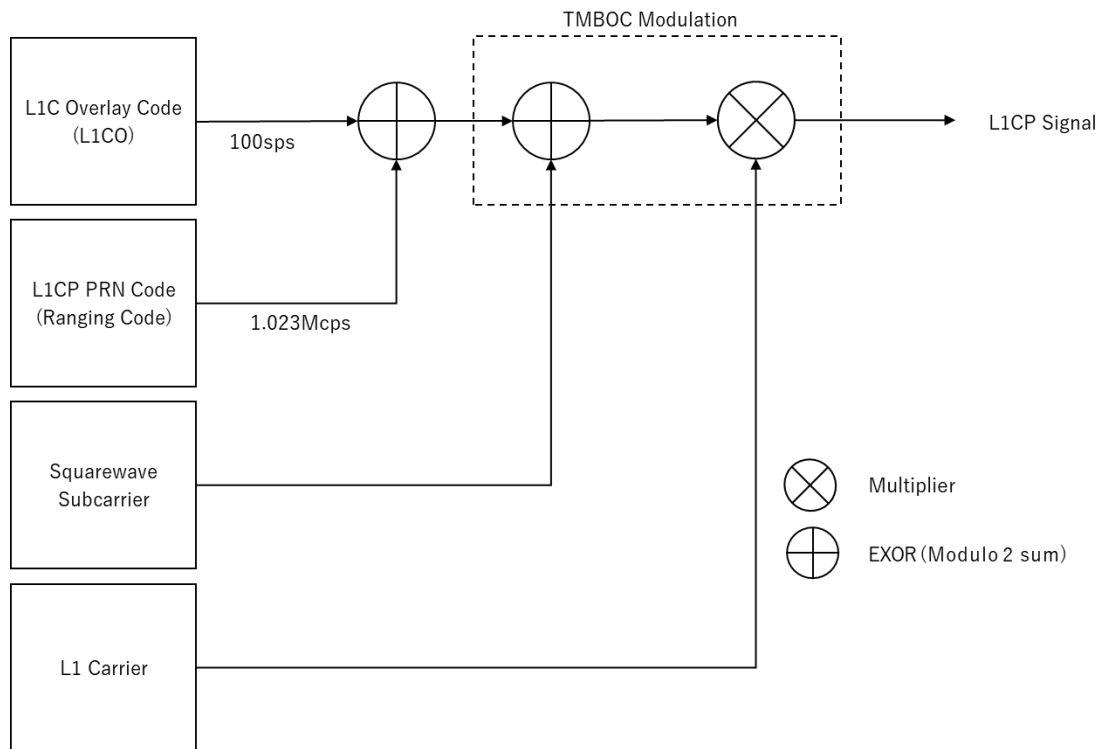
Figure 3.1.3-3 L1CP Modulation
