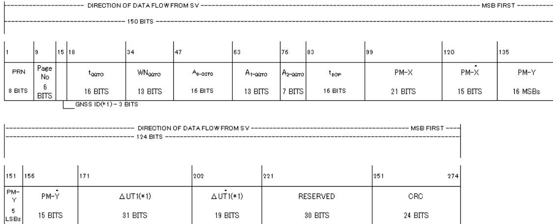
Figure 4.2.2-5 Subframe 3, Page 2: GGTO and EOP Format
