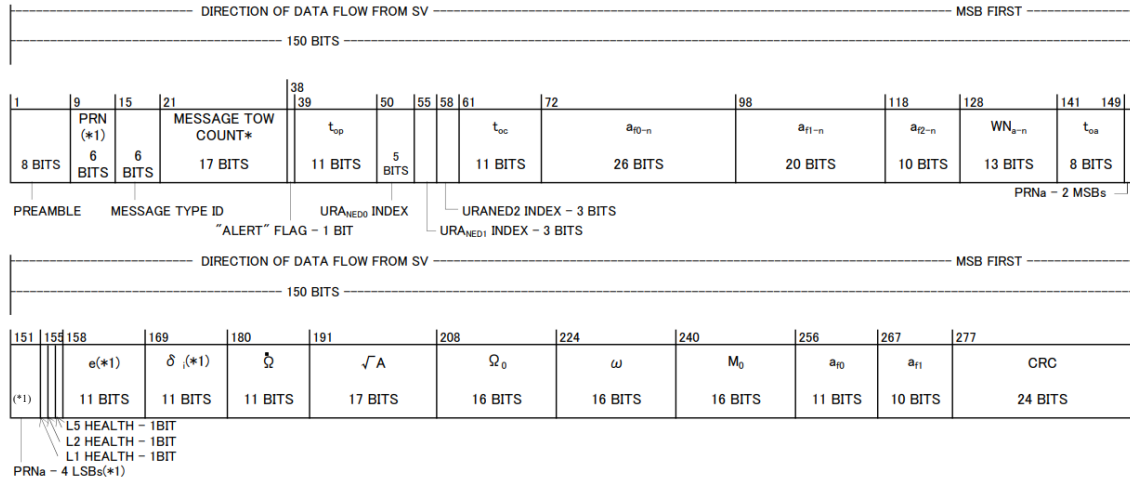
Figure 4.3.2-13 Message Type 37: Clock and Midi Almanac Format
