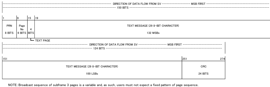
Figure 4.2.2-9 Subframe 3, Page 6: Text Message Format
