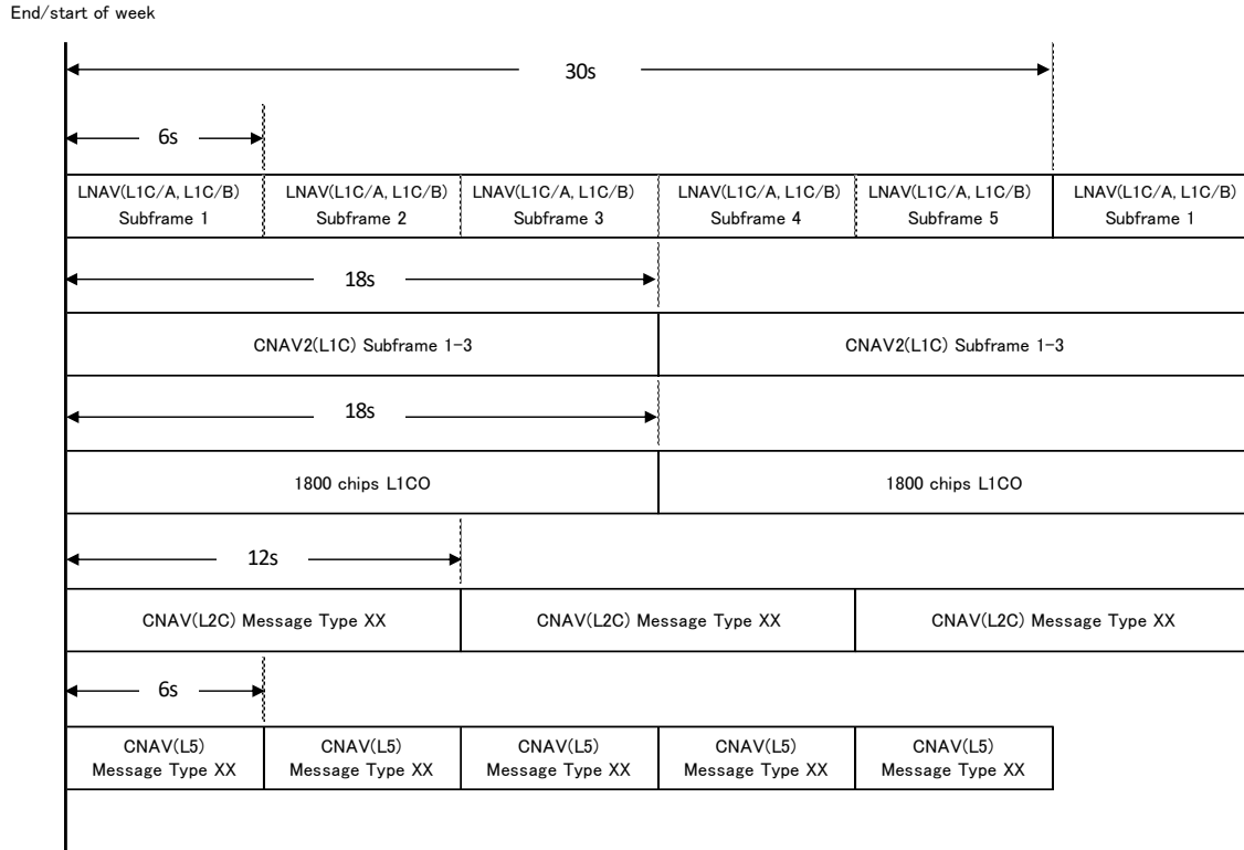
Figure 3.1.3-8 Navigation Message Timing
