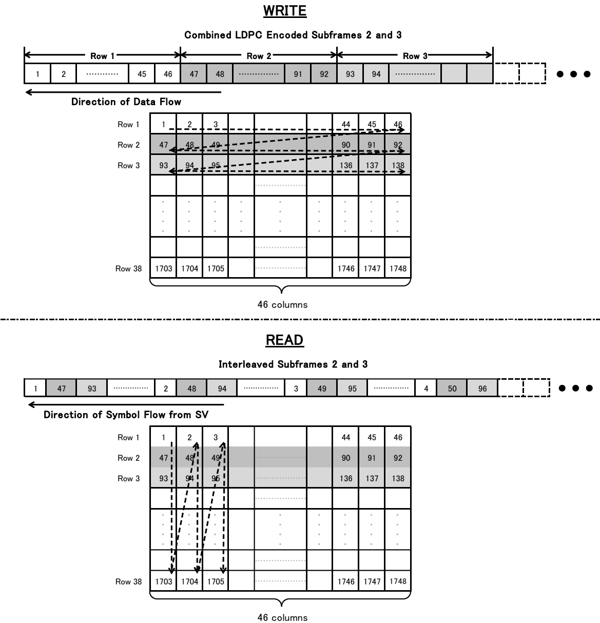
Figure 4.2.1-4 Interleaving
