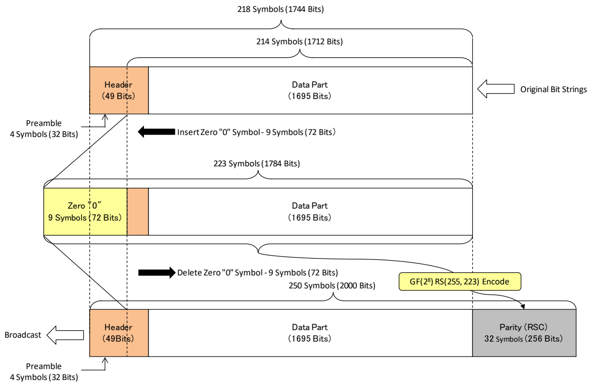
Figure 4.1.3-1 Compact SSR STEC correction message structure
