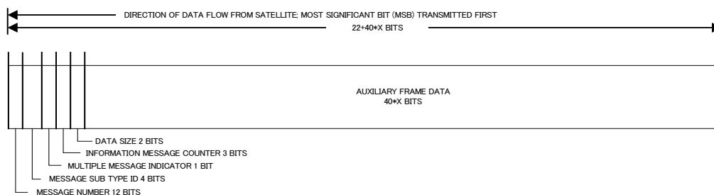
Figure 4.1.2-12 Compact SSR Service Information Message structure
