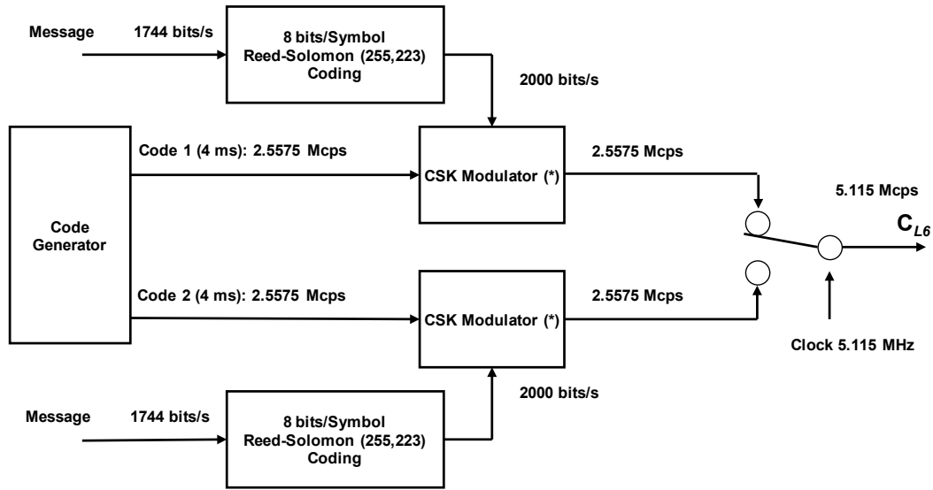
Figure 3.1.3-2 L62 Signal structure
