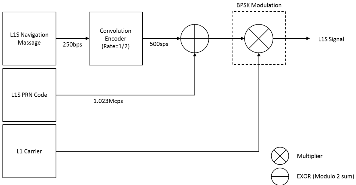
Figure 3.1.3-1 L1S Modulation
